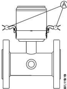
MAG 8000 CT user sealing (A) - compact
