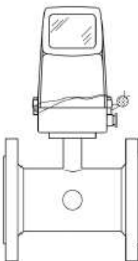
Compact version with 1 wire
